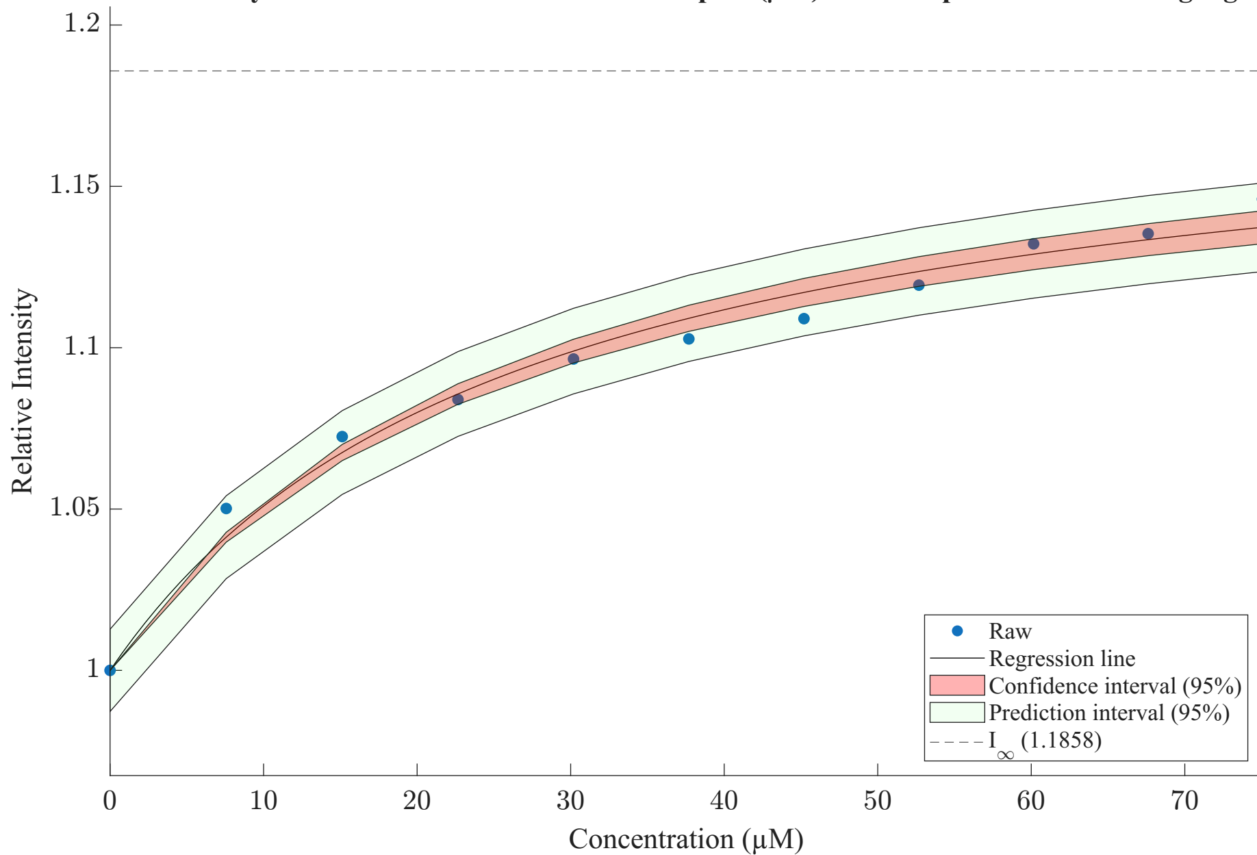
Relative intensity as a function of concentration of lipids (μM) for t1r rep3 - Statistics fitting algorithm
